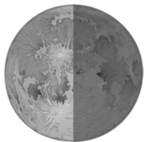
Last Quarter
