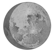
Waxing Gibbous
