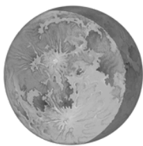
Waning Gibbous
