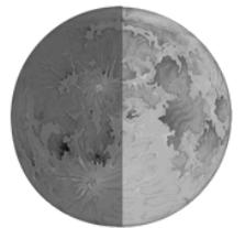
First Quarter
