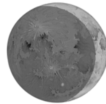
Waxing Crescent
